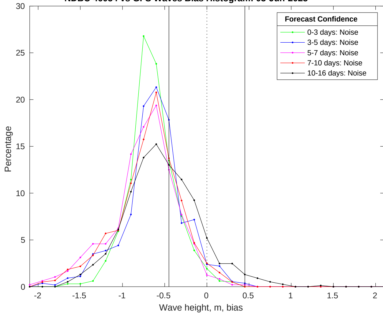
NDBC 46054 vs GFS Waves Bias Histogram: 03-Jun-2025
