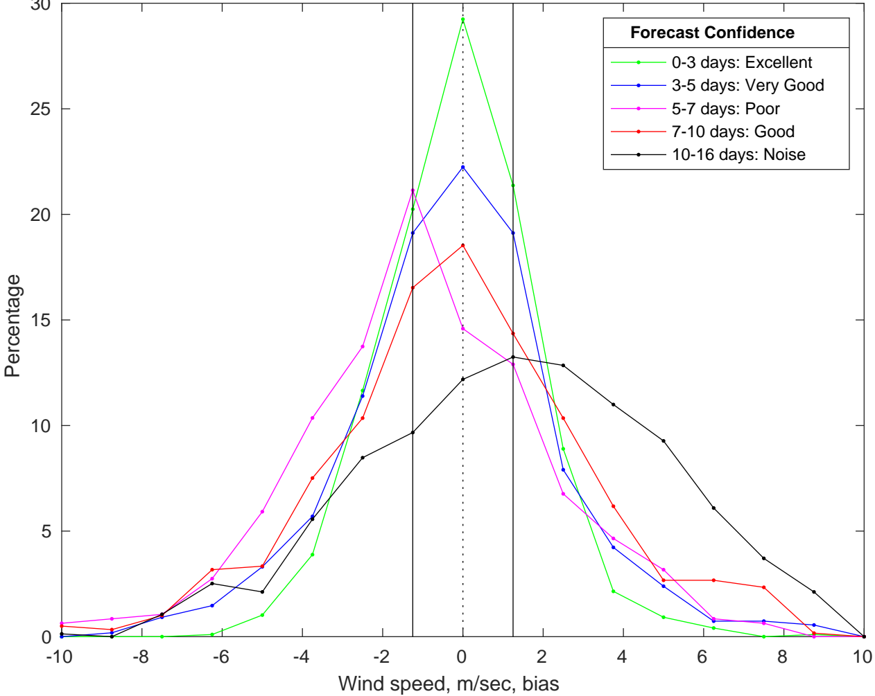
NDBC 46054 vs GFS Winds Bias Histogram: 03-Jun-2025
