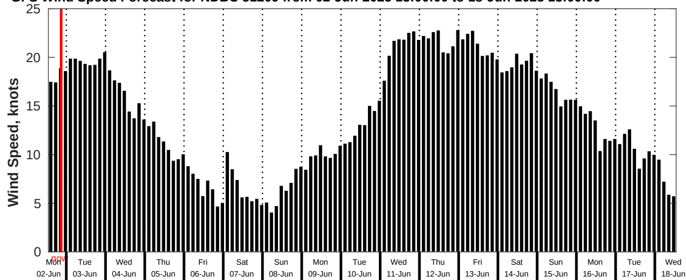
GFS Wind Speed Forecast for NDBC 51209 from 02-Jun-2025 13:00:00 to 18-Jun-2025 13:00:00
