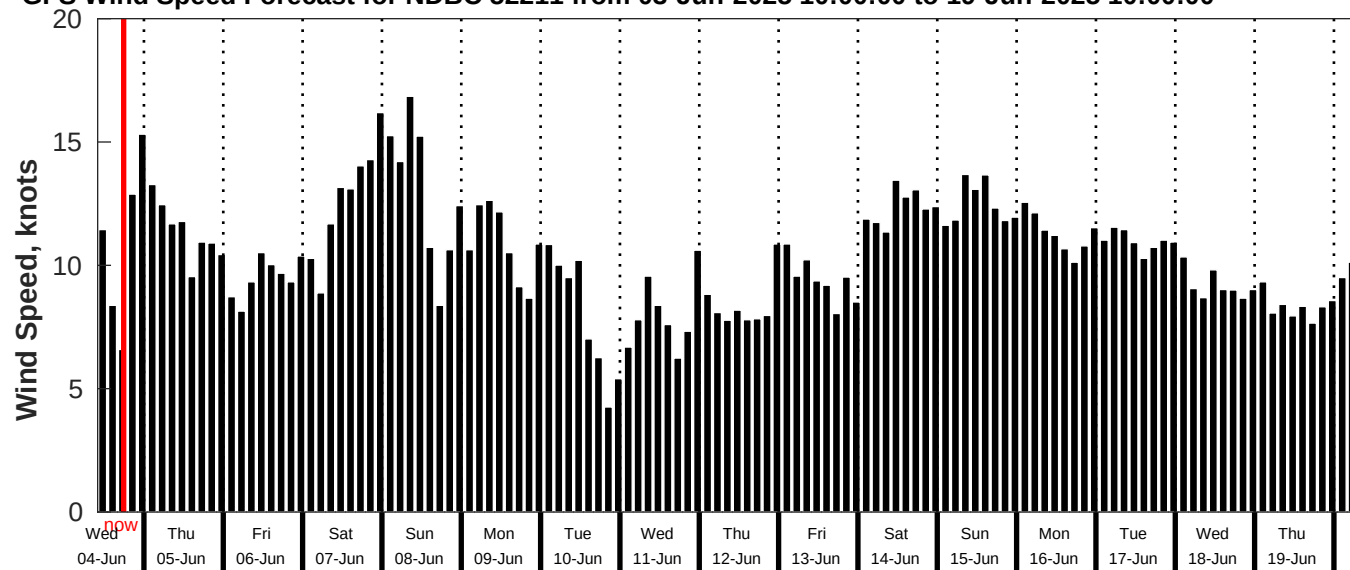
GFS Wind Speed Forecast for NDBC 52211 from 03-Jun-2025 10:00:00 to 19-Jun-2025 10:00:00
