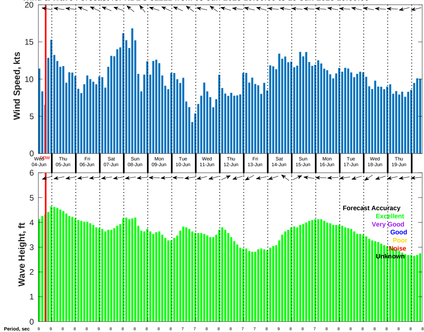
Wind & Wave Forecast for NDBC 52211 from 03-Jun-2025 10:00:00 to 19-Jun-2025 10:00:00
