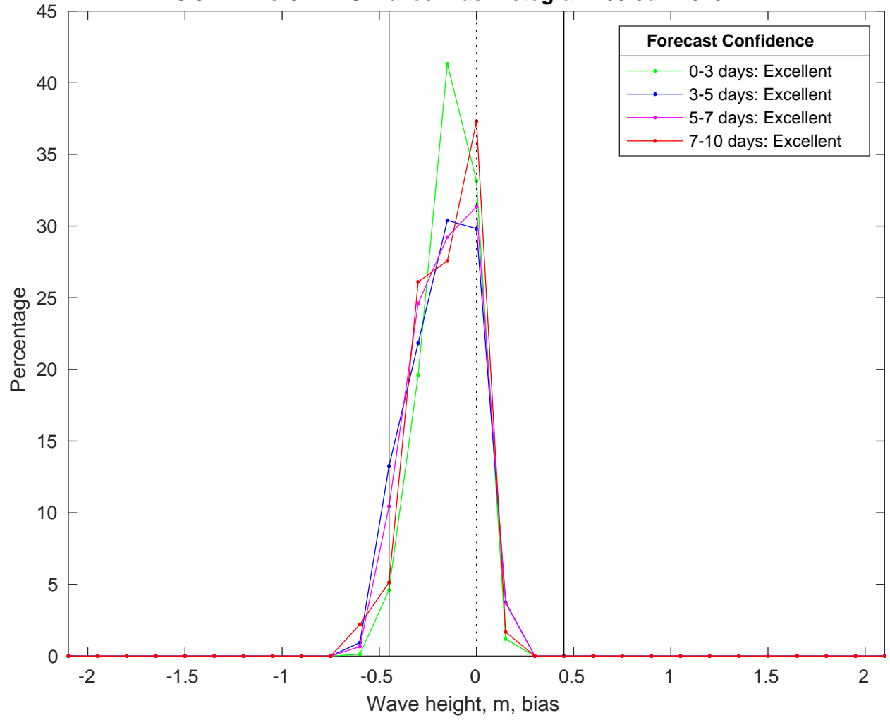
NDBC 52212 vs CMEMS Waves Bias Histogram: 03-Jun-2025
