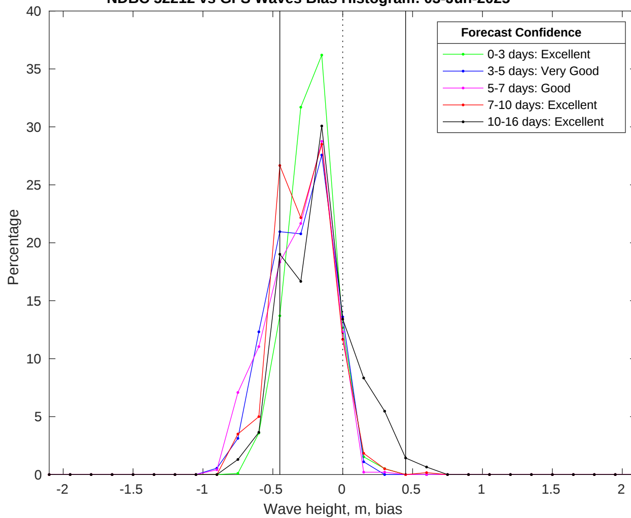
NDBC 52212 vs GFS Waves Bias Histogram: 03-Jun-2025
