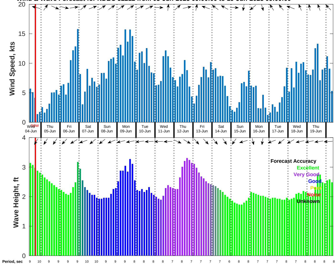
Wind & Wave Forecast for NDBC 52212 from 03-Jun-2025 09:00:00 to 19-Jun-2025 09:00:00
