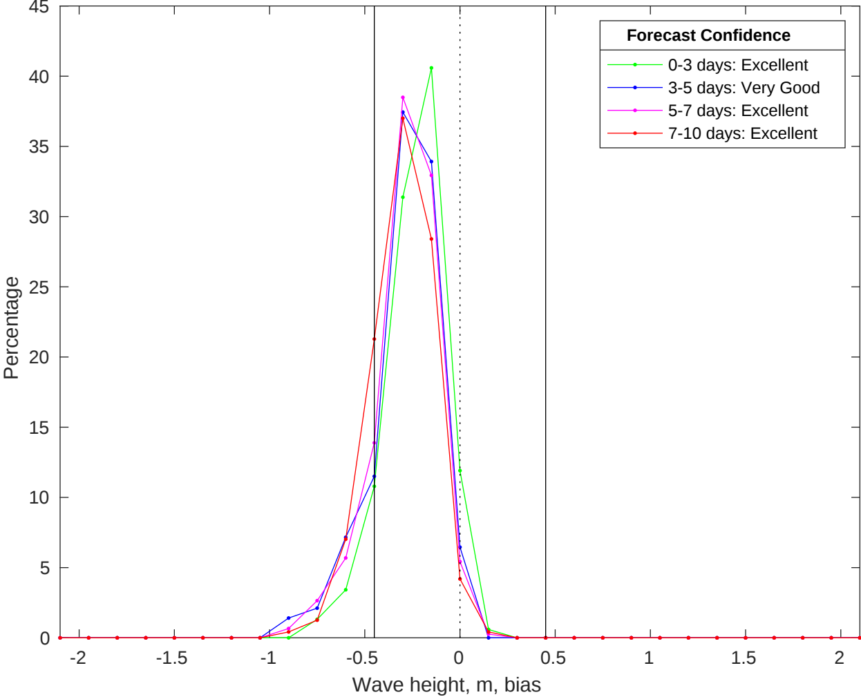
NDBC 52213 vs CMEMS Waves Bias Histogram: 03-Jun-2025
