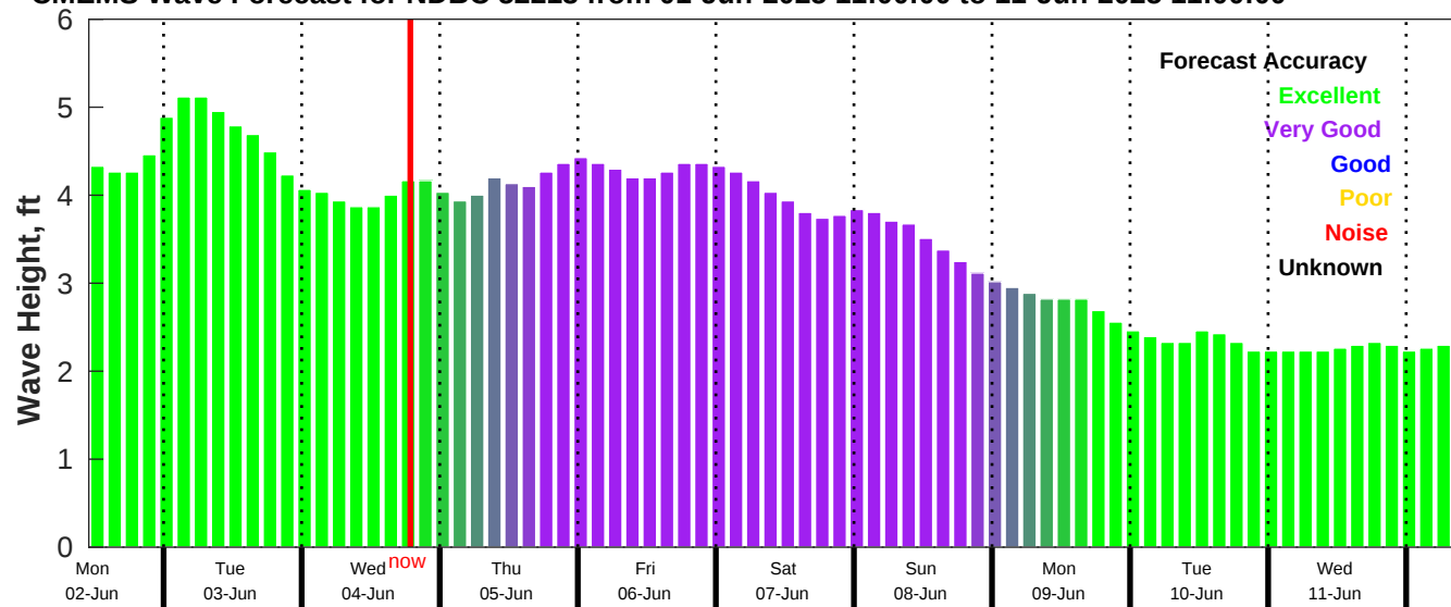
CMEMS Wave Forecast for NDBC 52213 from 01-Jun-2025 11:00:00 to 11-Jun-2025 11:00:00
