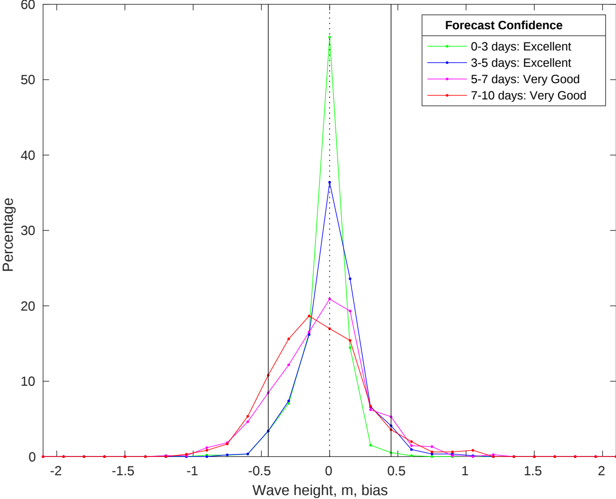
NDBC 41004 vs CMEMS Waves Bias Histogram: 04-Jun-2025
