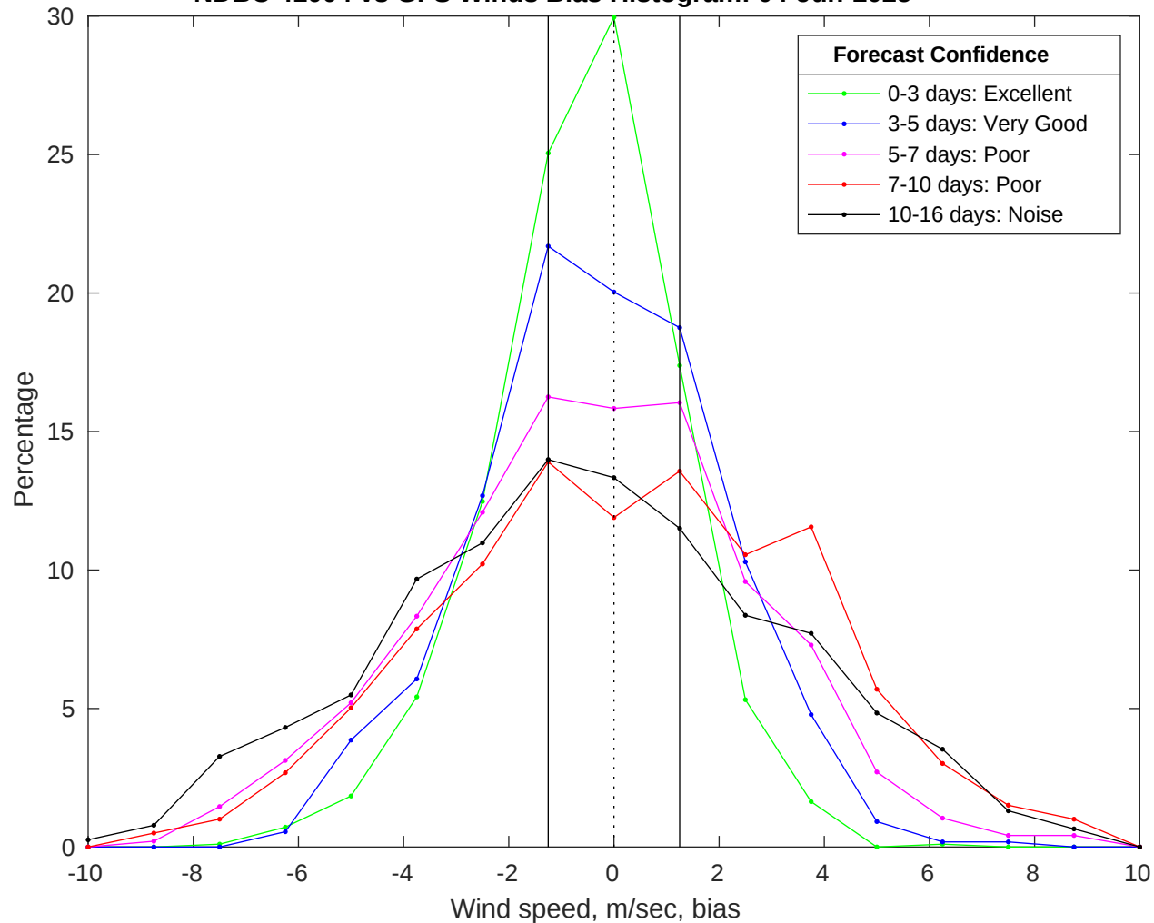
NDBC 41004 vs GFS Winds Bias Histogram: 04-Jun-2025
