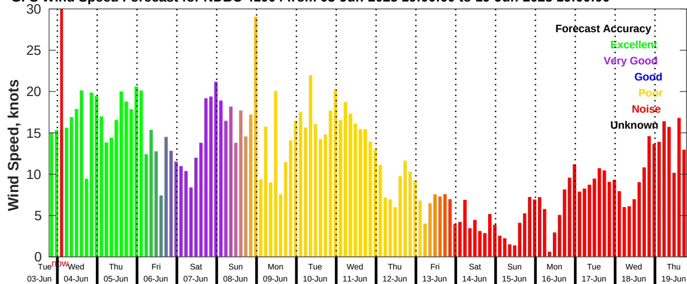
GFS Wind Speed Forecast for NDBC 41004 from 03-Jun-2025 19:00:00 to 19-Jun-2025 19:00:00
