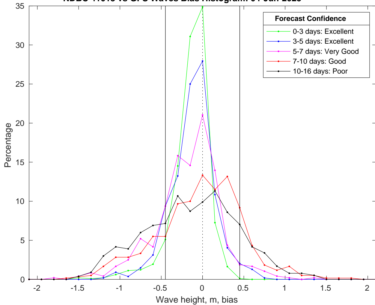
NDBC 41013 vs GFS Waves Bias Histogram: 04-Jun-2025
