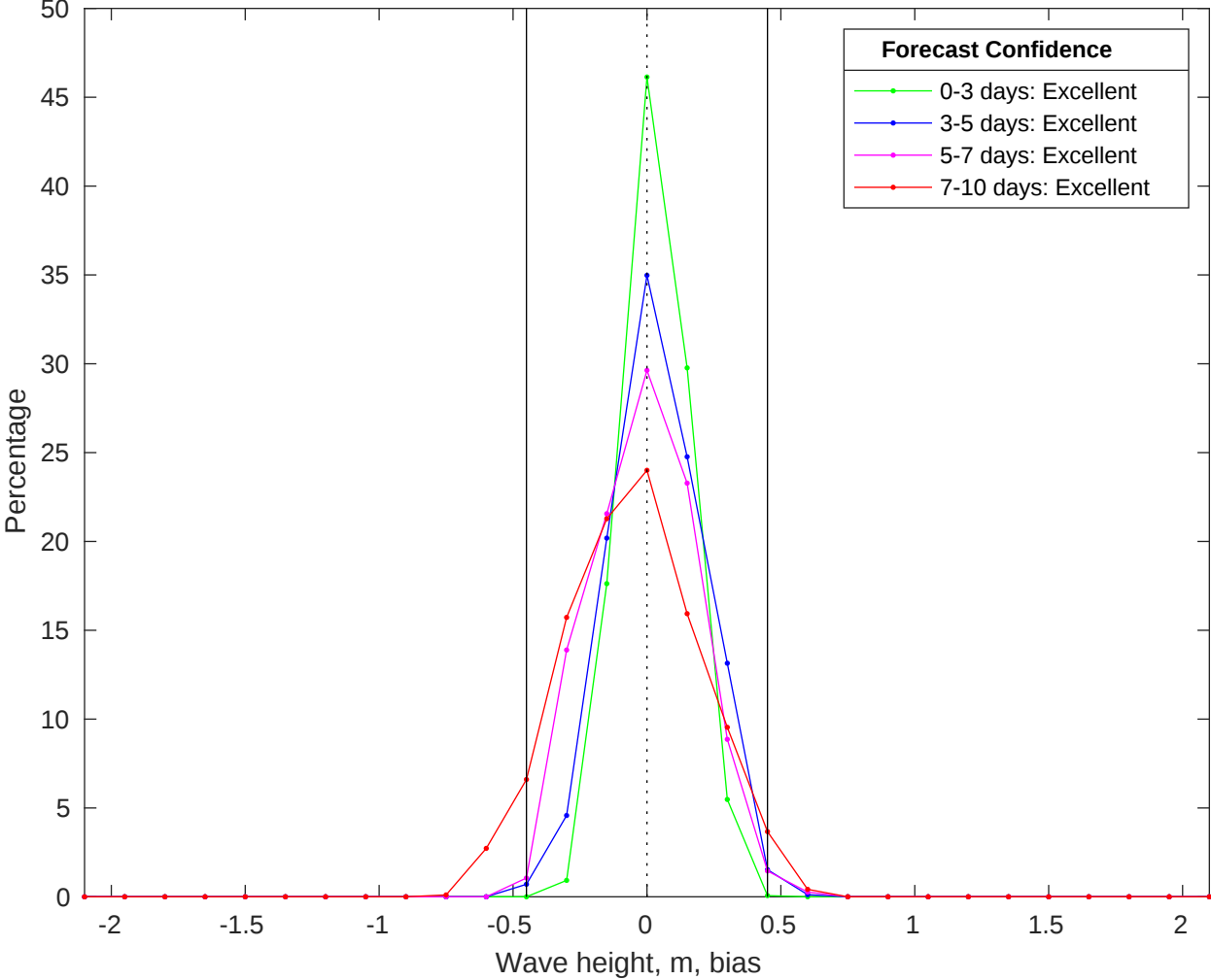
NDBC 41040 vs CMEMS Waves Bias Histogram: 04-Jun-2025
