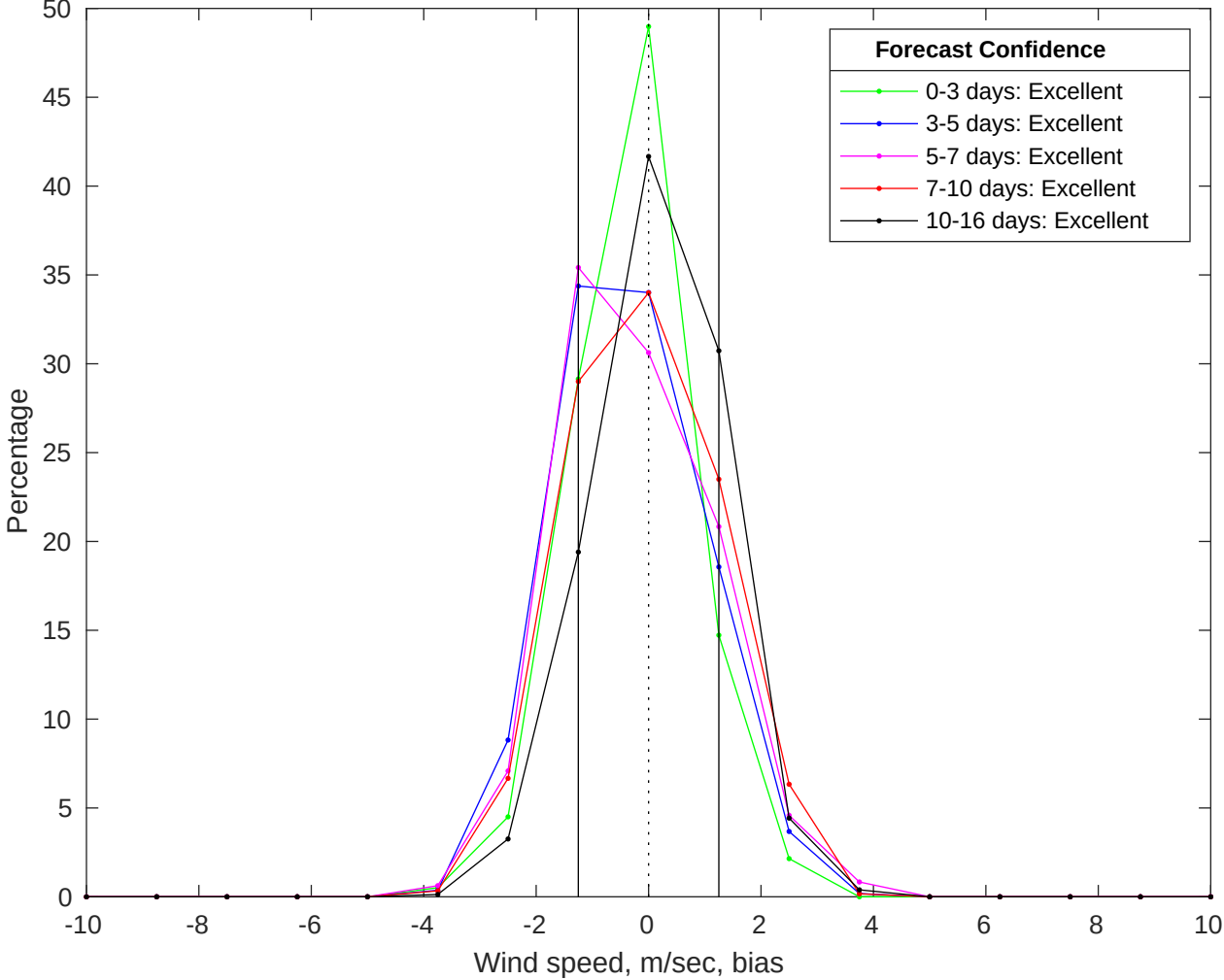
NDBC 41040 vs GFS Winds Bias Histogram: 04-Jun-2025
