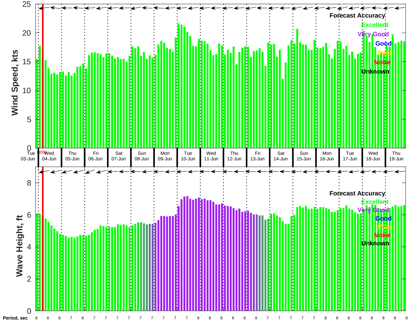
Wind & Wave Forecast for NDBC 41040 from 03-Jun-2025 21:00:00 to 19-Jun-2025 21:00:00
