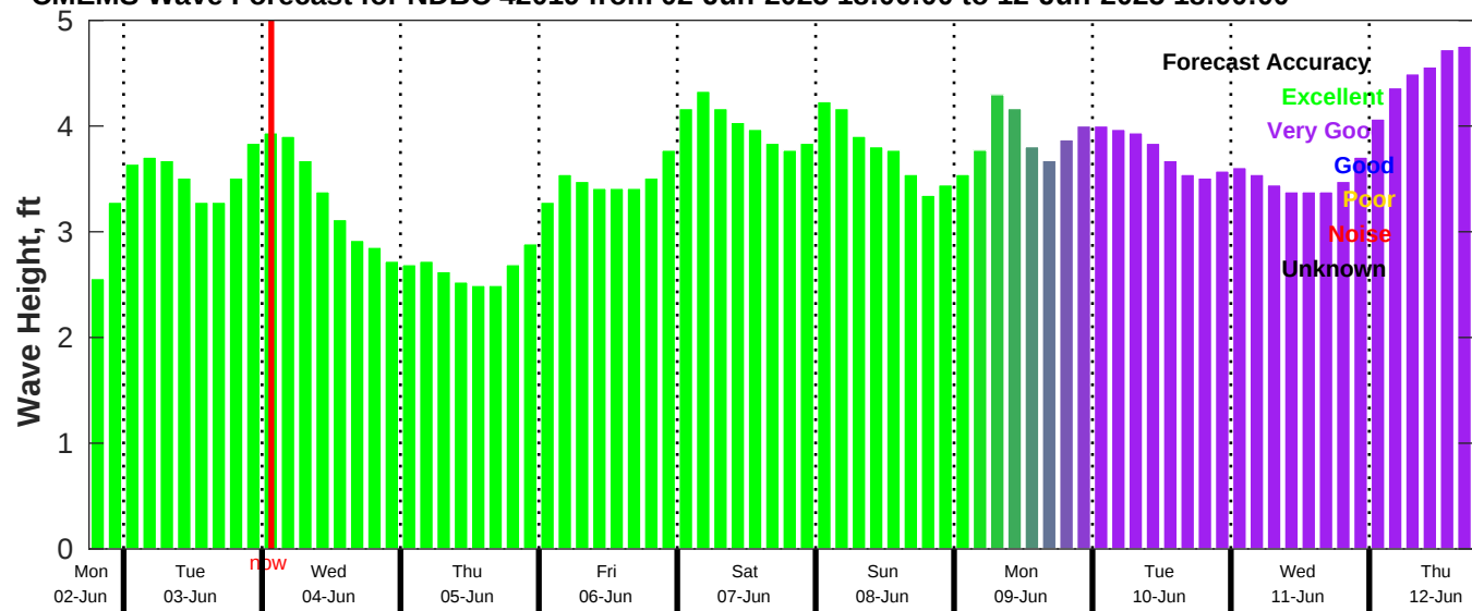
CMEMS Wave Forecast for NDBC 42019 from 02-Jun-2025 18:00:00 to 12-Jun-2025 18:00:00
