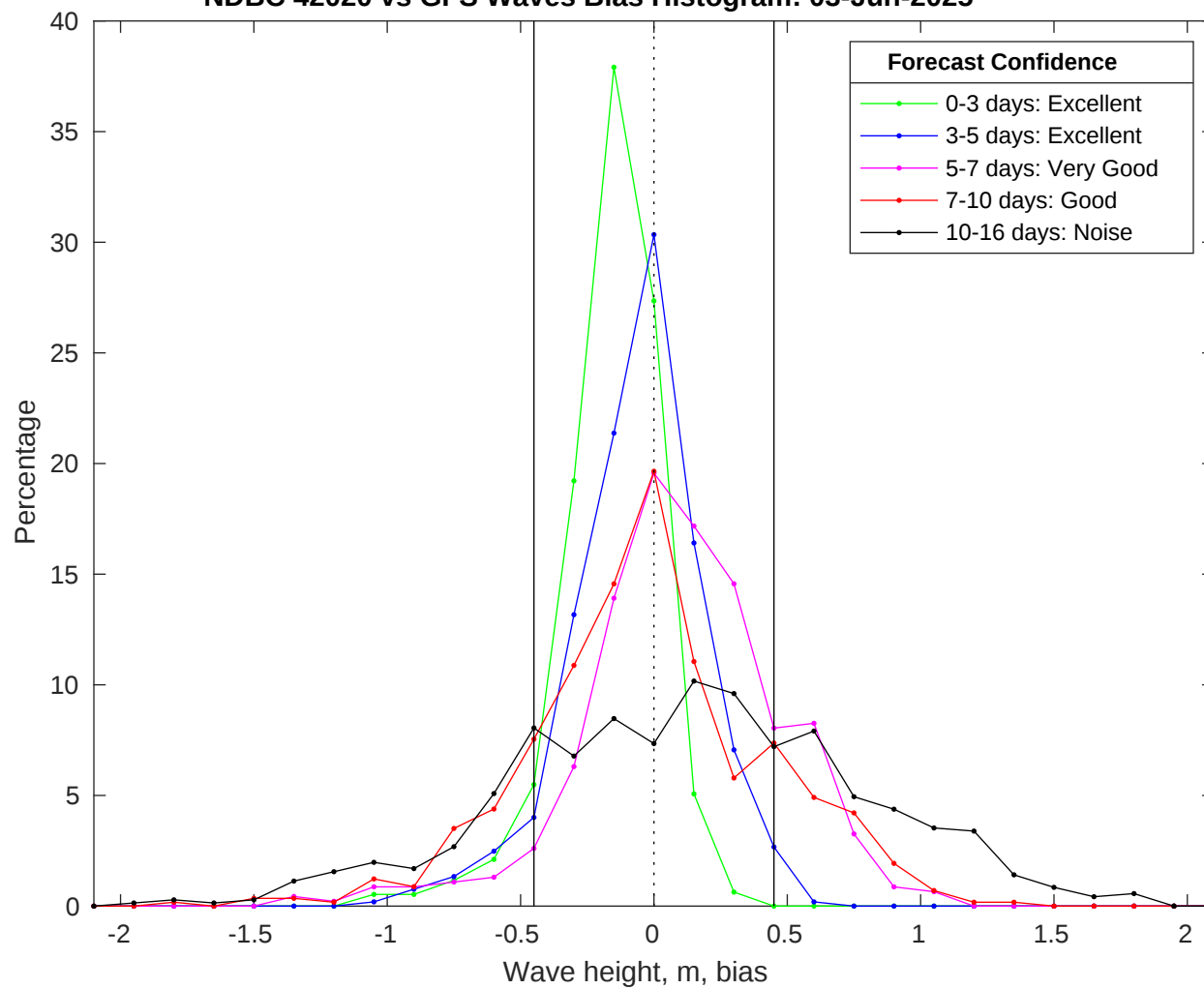
NDBC 42020 vs GFS Waves Bias Histogram: 03-Jun-2025
