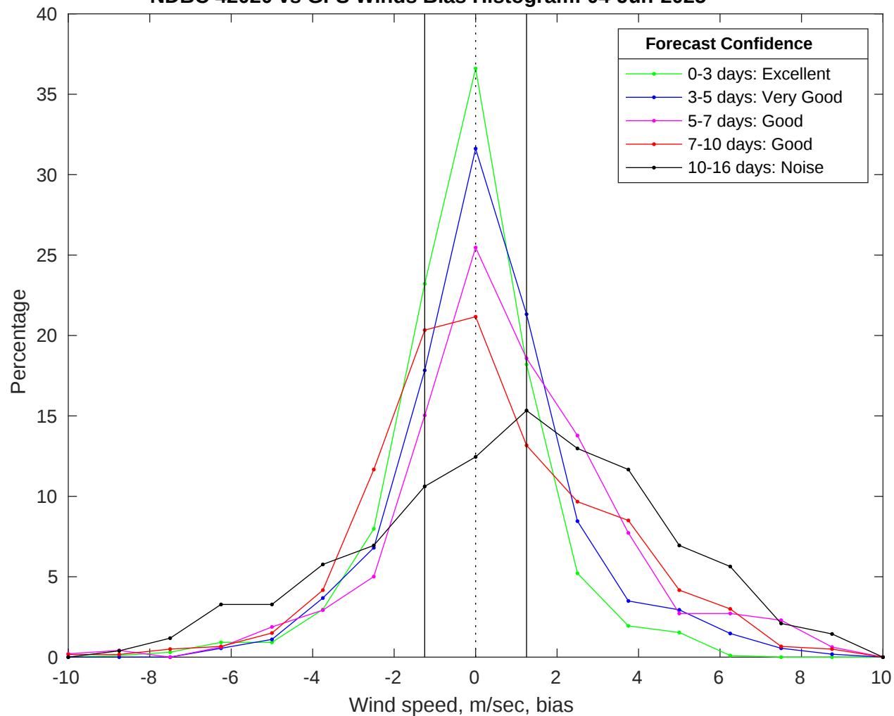
NDBC 42020 vs GFS Winds Bias Histogram: 04-Jun-2025
