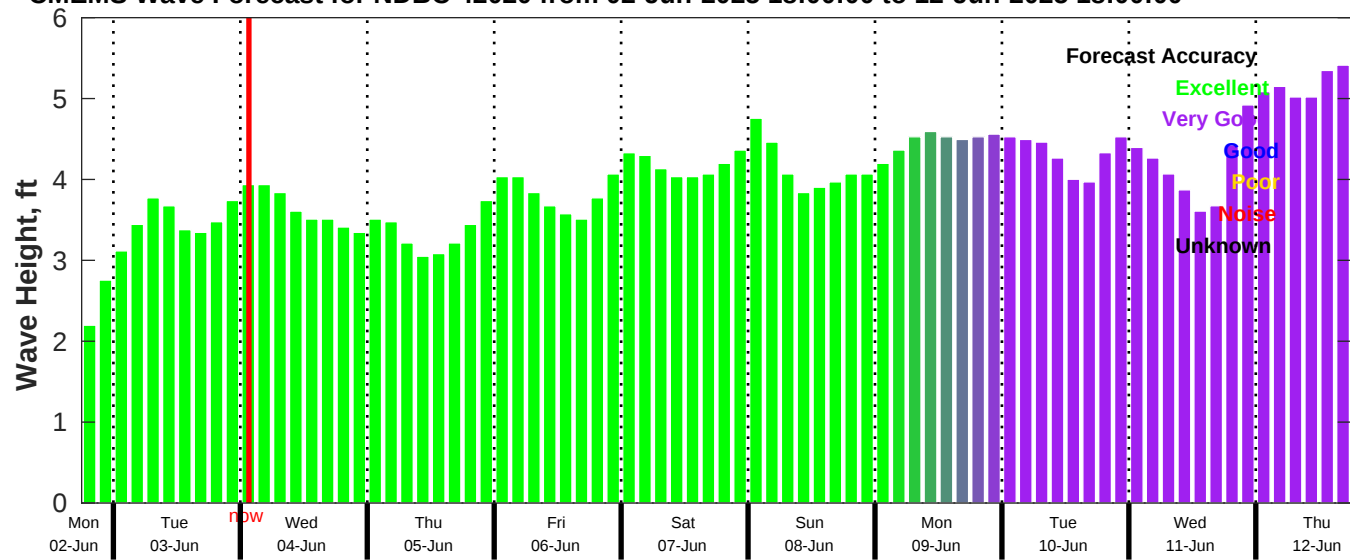
CMEMS Wave Forecast for NDBC 42020 from 02-Jun-2025 18:00:00 to 12-Jun-2025 18:00:00
