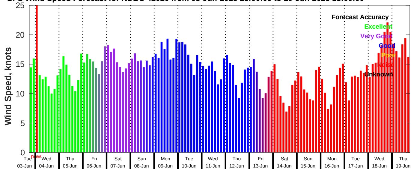
GFS Wind Speed Forecast for NDBC 42020 from 03-Jun-2025 18:00:00 to 19-Jun-2025 18:00:00
