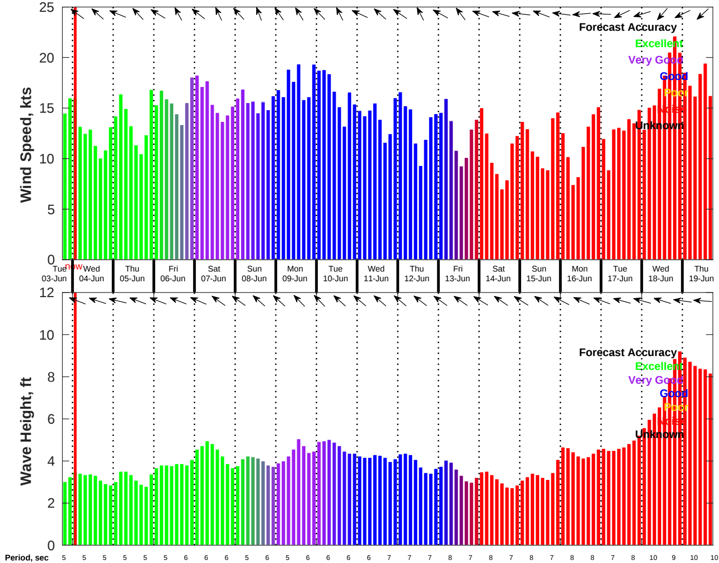
Wind & Wave Forecast for NDBC 42020 from 03-Jun-2025 18:00:00 to 19-Jun-2025 18:00:00
