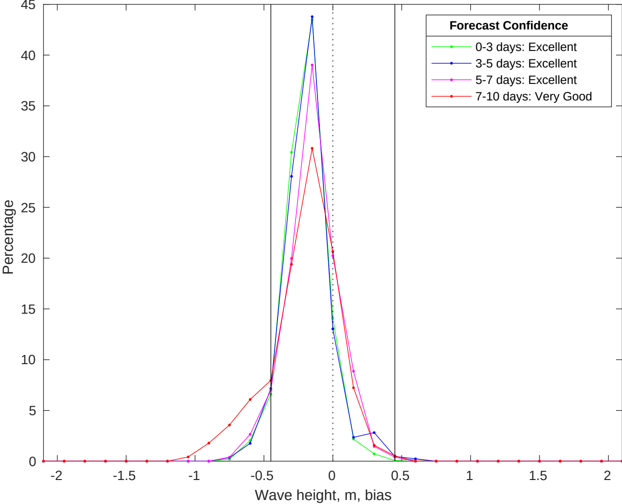
NDBC 42035 vs CMEMS Waves Bias Histogram: 04-Jun-2025
