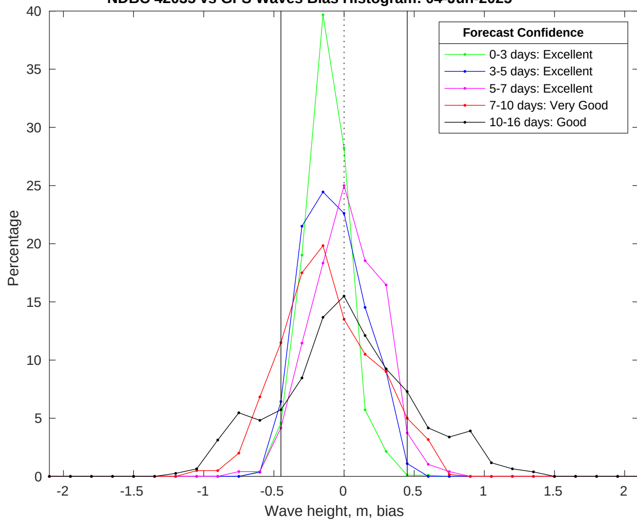
NDBC 42035 vs GFS Waves Bias Histogram: 04-Jun-2025
