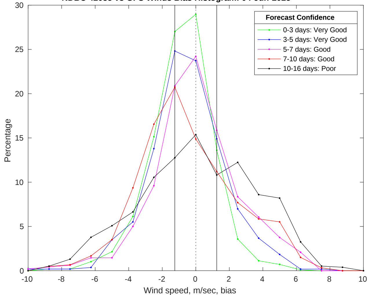
NDBC 42035 vs GFS Winds Bias Histogram: 04-Jun-2025
