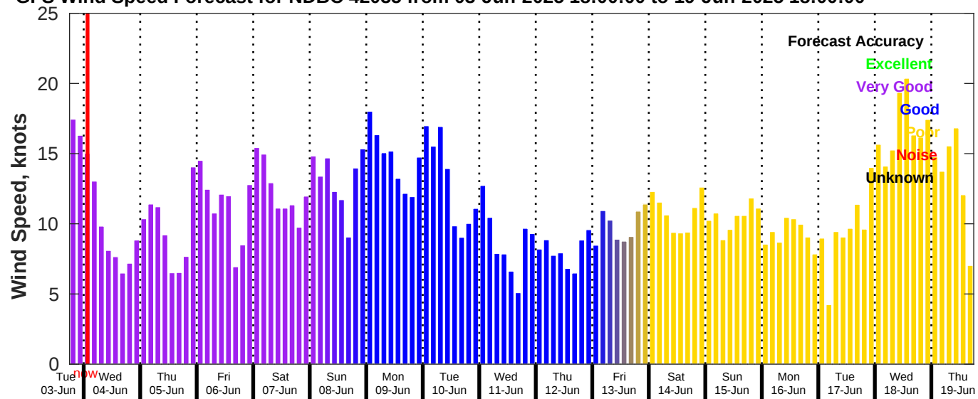
GFS Wind Speed Forecast for NDBC 42035 from 03-Jun-2025 18:00:00 to 19-Jun-2025 18:00:00
