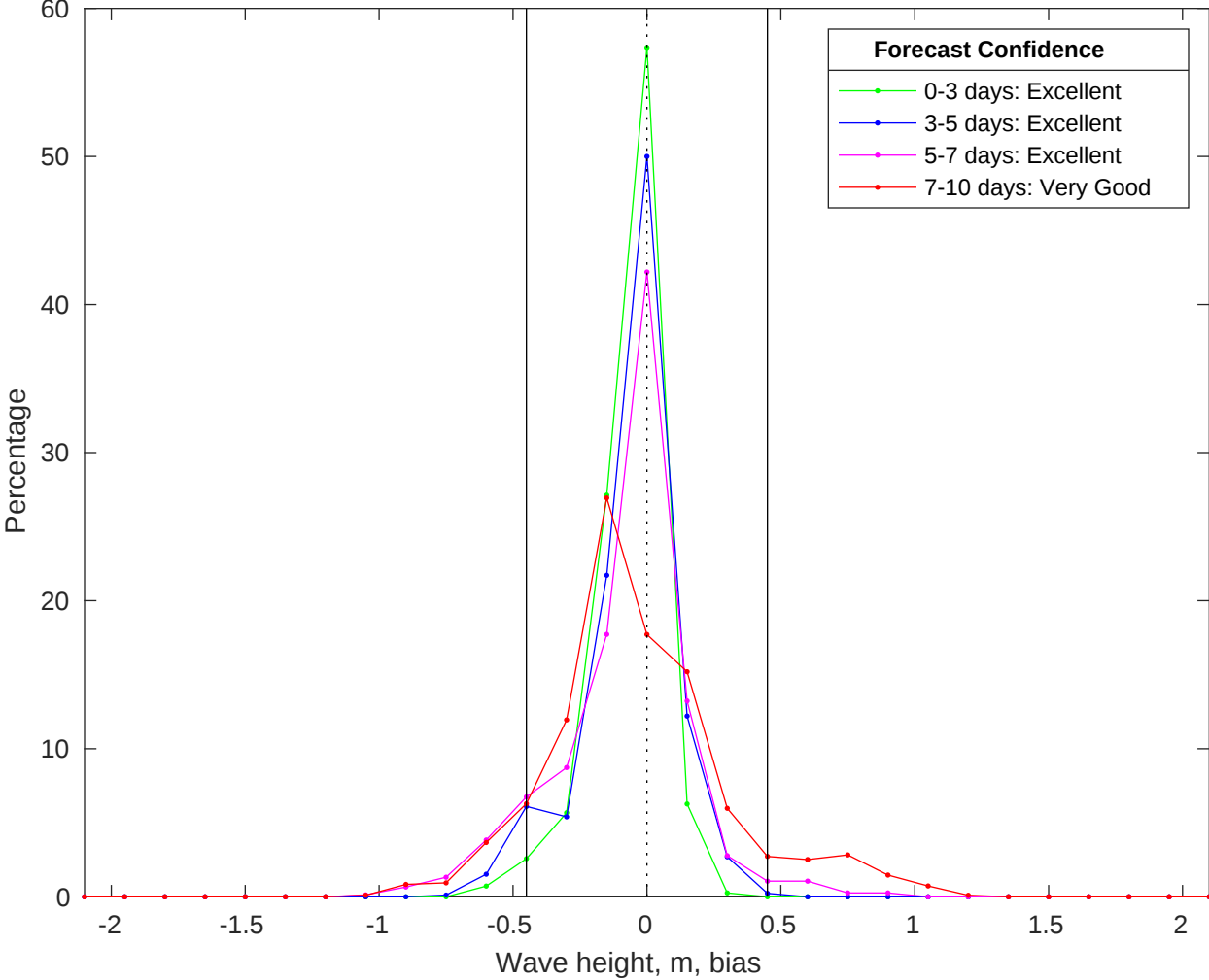
NDBC 42036 vs CMEMS Waves Bias Histogram: 04-Jun-2025
