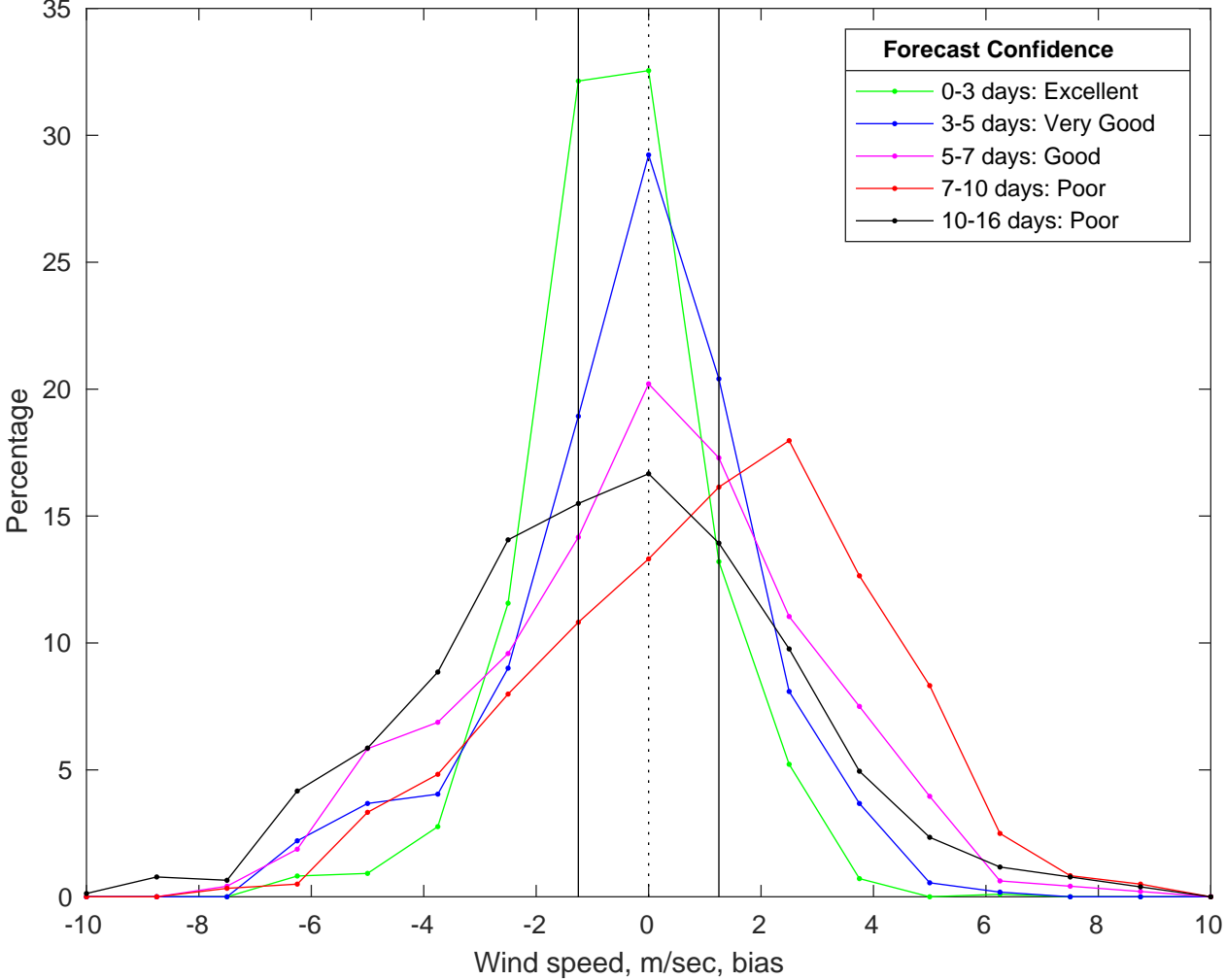
NDBC 42036 vs GFS Winds Bias Histogram: 04-Jun-2025
