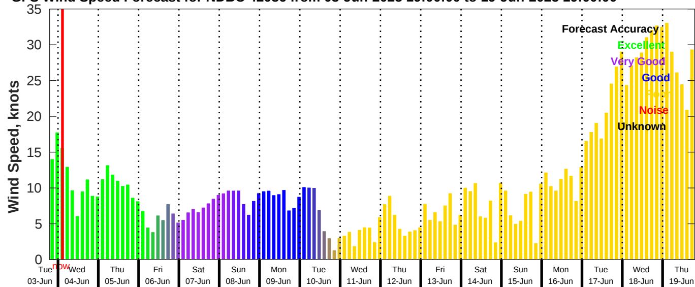
GFS Wind Speed Forecast for NDBC 42036 from 03-Jun-2025 19:00:00 to 19-Jun-2025 19:00:00
