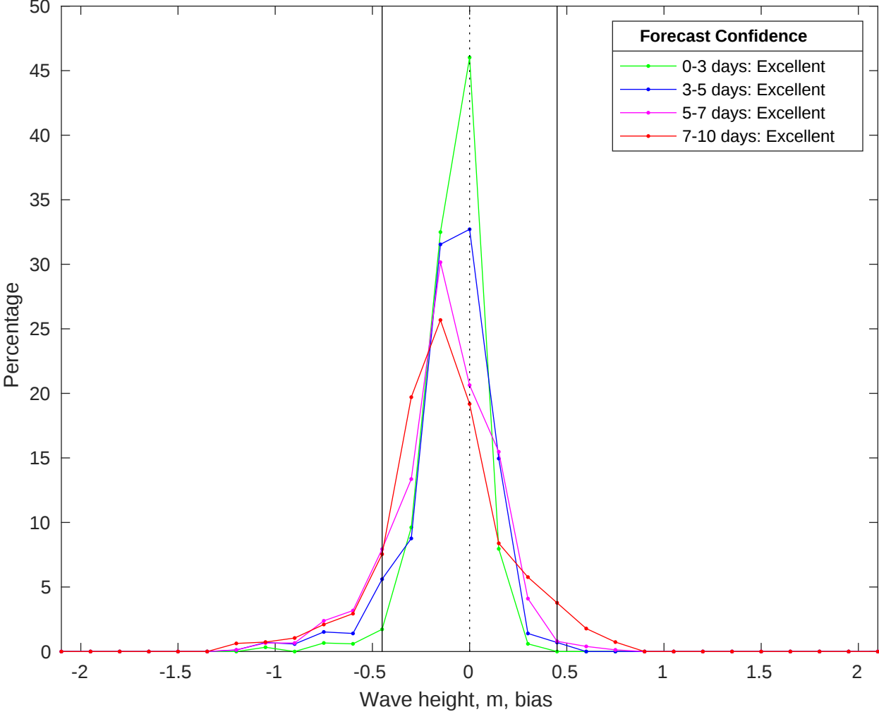
NDBC 42040 vs CMEMS Waves Bias Histogram: 04-Jun-2025
