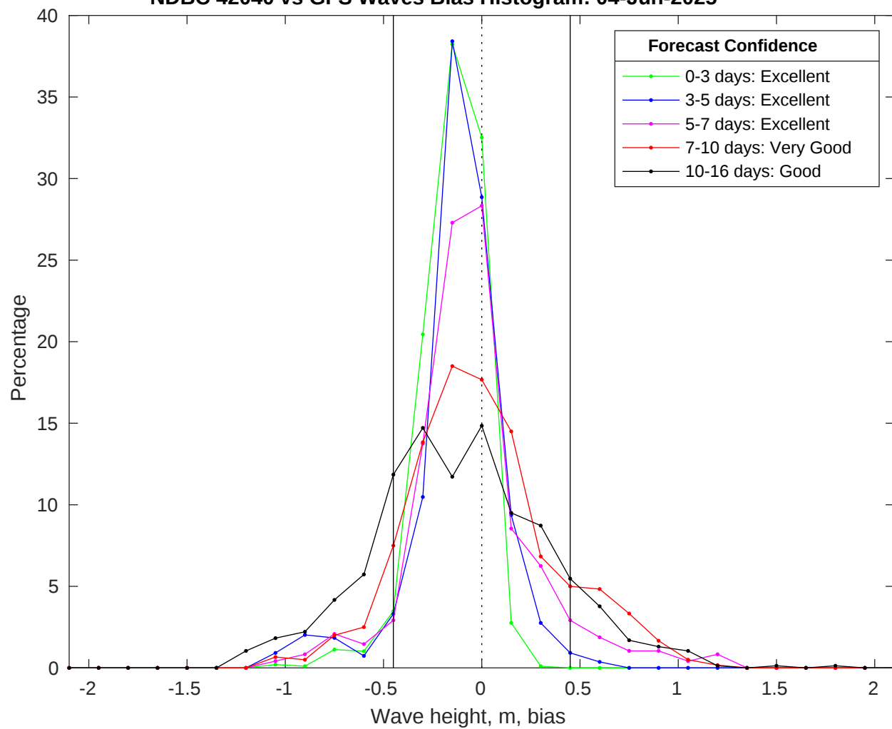
NDBC 42040 vs GFS Waves Bias Histogram: 04-Jun-2025
