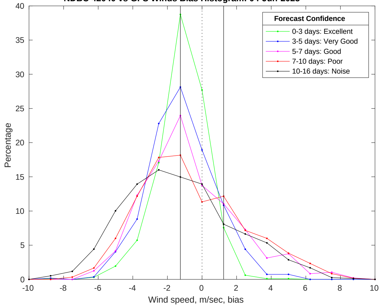
NDBC 42040 vs GFS Winds Bias Histogram: 04-Jun-2025
