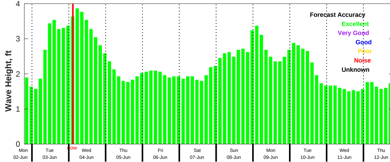
CMEMS Wave Forecast for NDBC 42040 from 02-Jun-2025 19:00:00 to 12-Jun-2025 19:00:00
