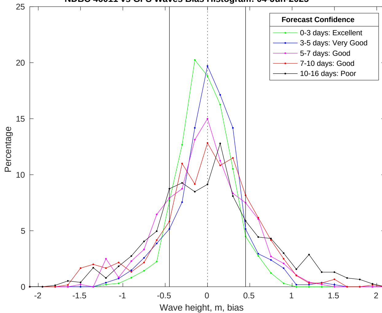
NDBC 46011 vs GFS Waves Bias Histogram: 04-Jun-2025
