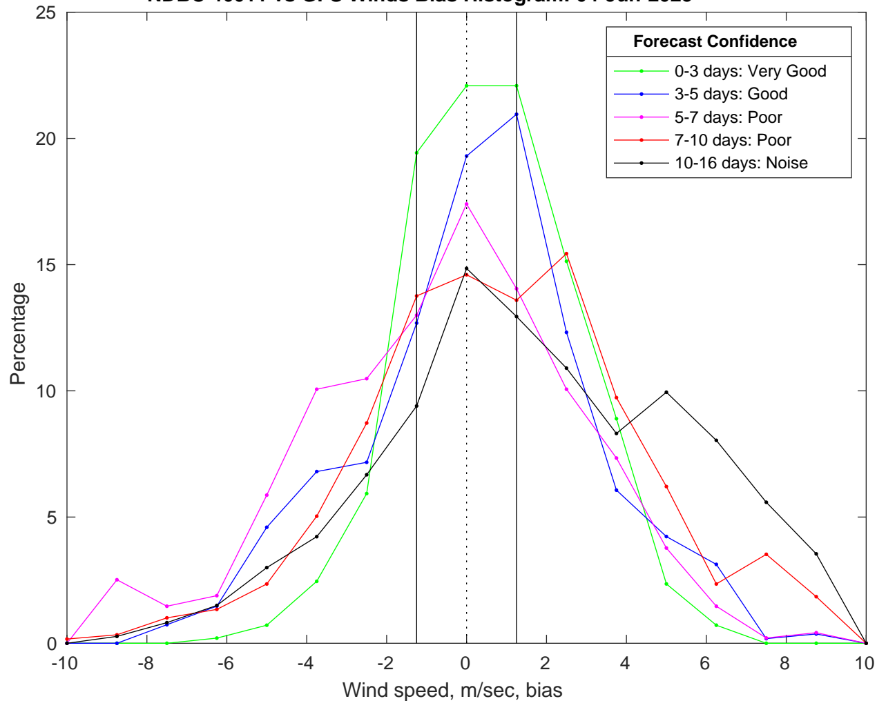
NDBC 46011 vs GFS Winds Bias Histogram: 04-Jun-2025
