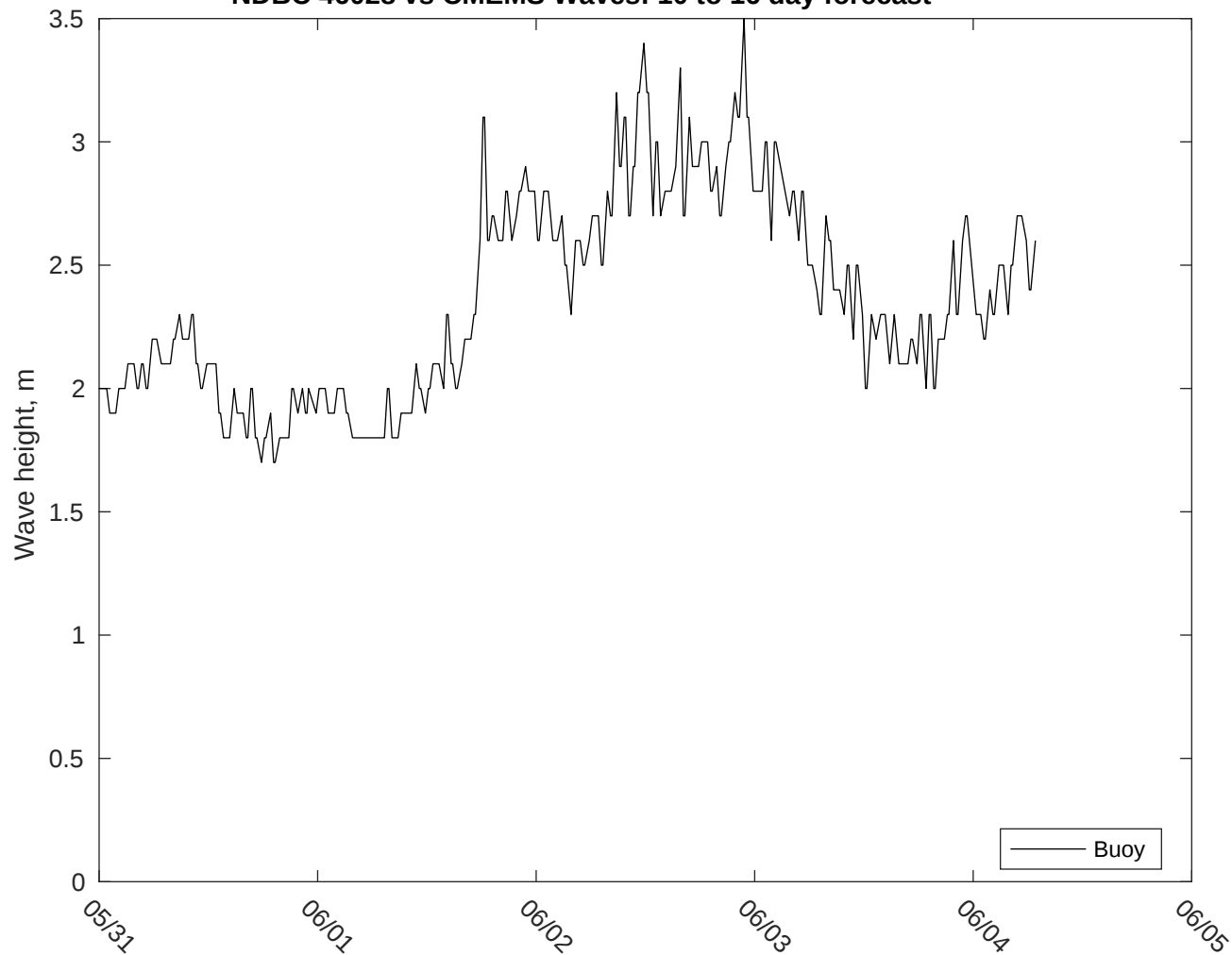
NDBC 46028 vs CMEMS Waves: 10 to 16 day forecast
