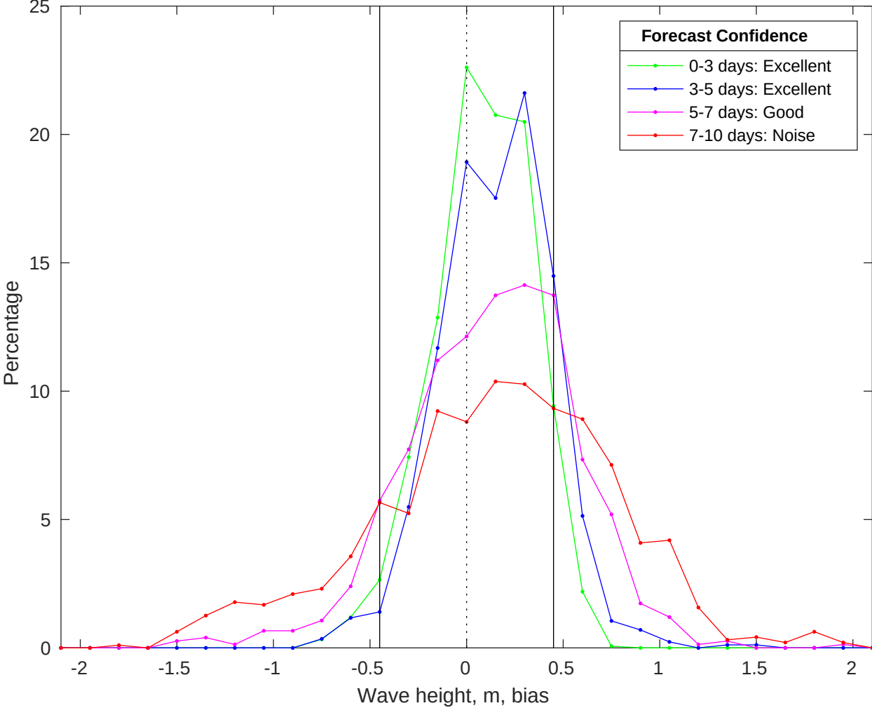
NDBC 46028 vs CMEMS Waves Bias Histogram: 04-Jun-2025
