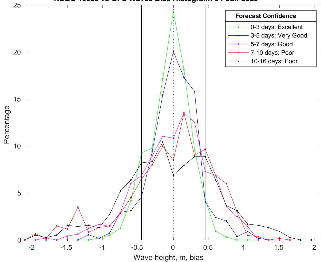
NDBC 46028 vs GFS Waves Bias Histogram: 04-Jun-2025
