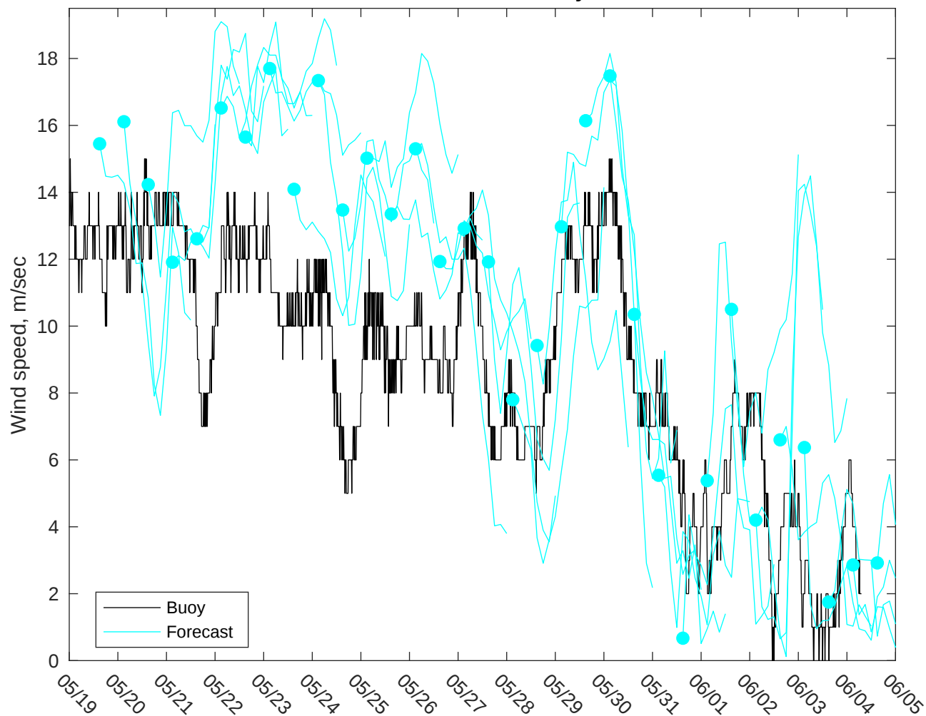
NDBC 46028 vs GFS Winds: 5 to 7 day forecast
