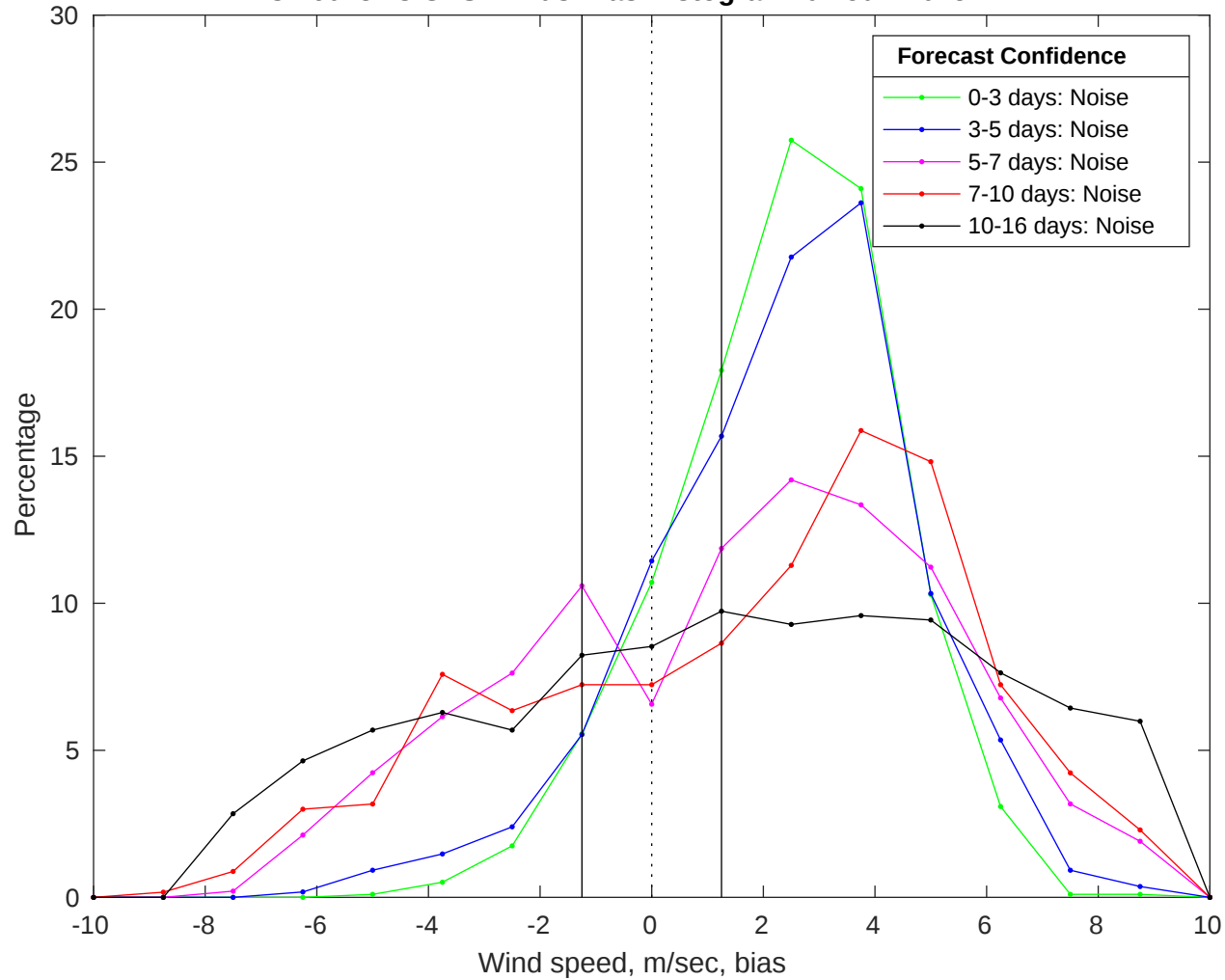
NDBC 46028 vs GFS Winds Bias Histogram: 04-Jun-2025
