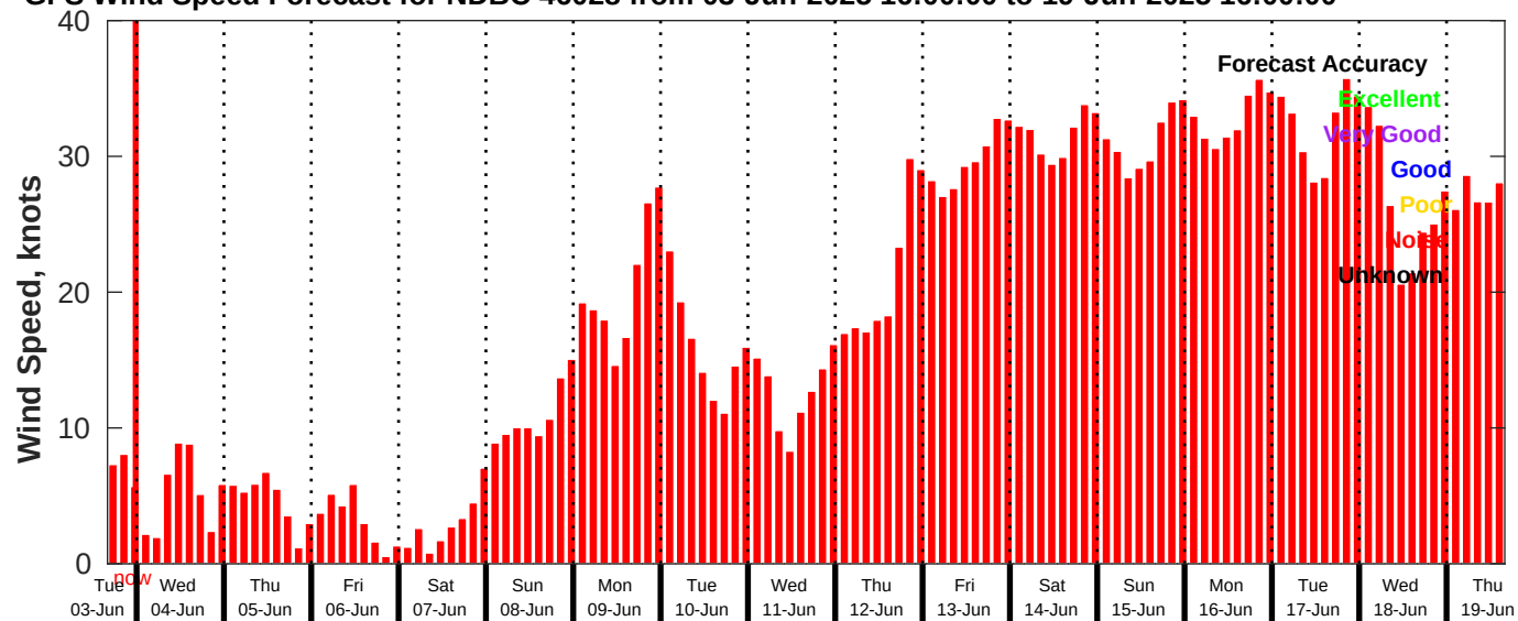
GFS Wind Speed Forecast for NDBC 46028 from 03-Jun-2025 16:00:00 to 19-Jun-2025 16:00:00
