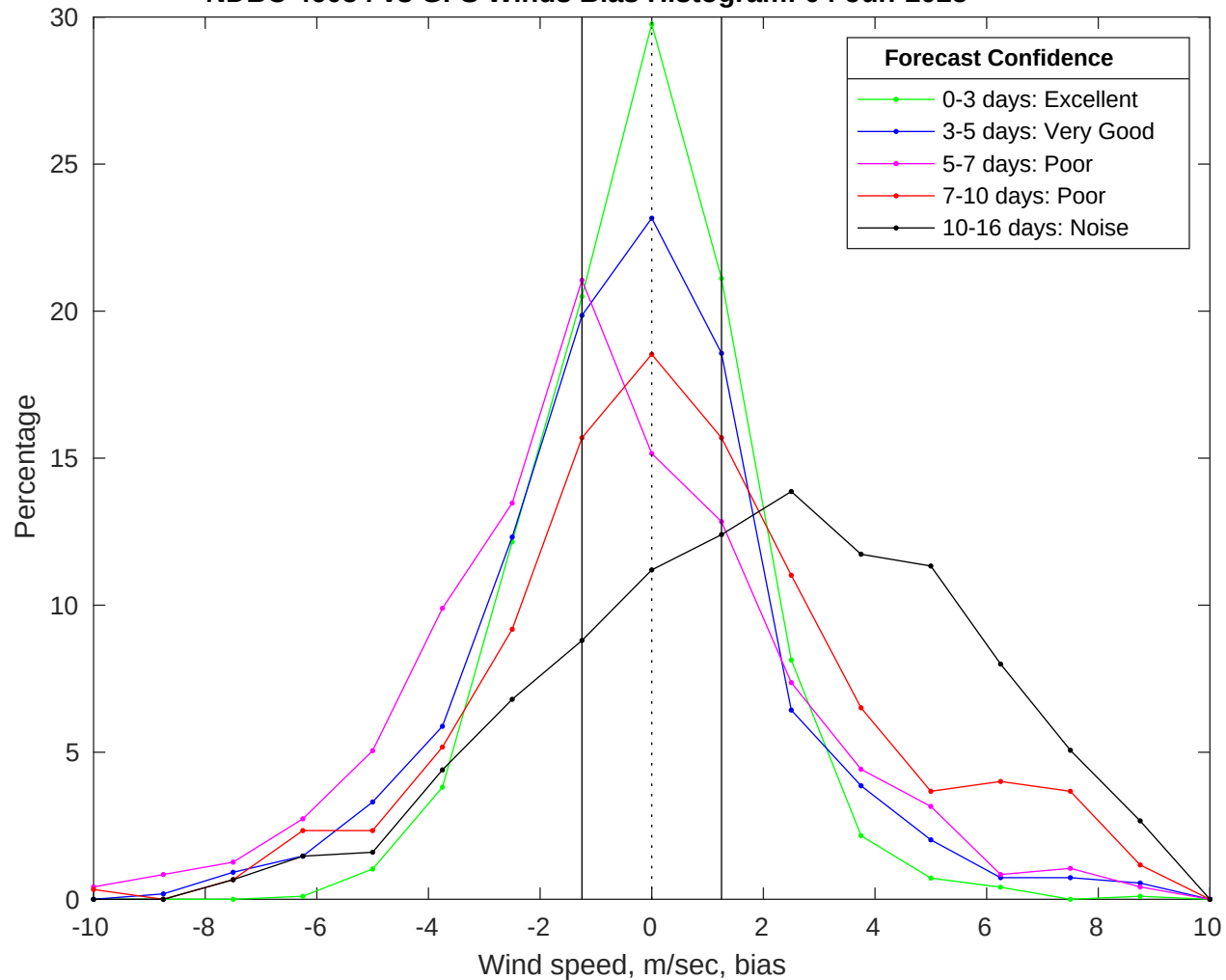
NDBC 46054 vs GFS Winds Bias Histogram: 04-Jun-2025
