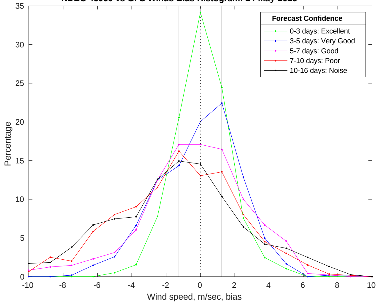
NDBC 46069 vs GFS Winds Bias Histogram: 24-May-2025
