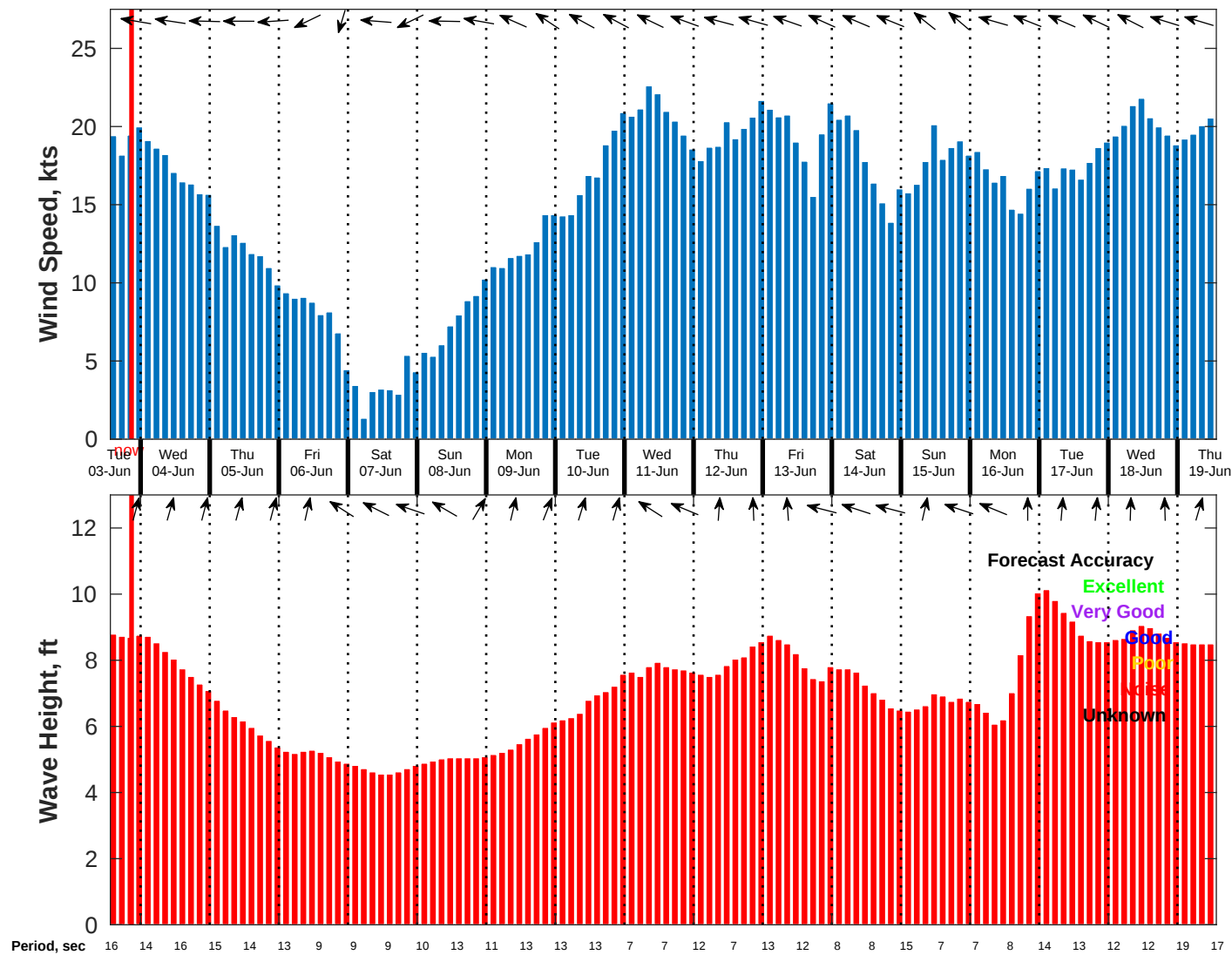
Wind & Wave Forecast for NDBC 51209 from 03-Jun-2025 13:00:00 to 19-Jun-2025 13:00:00
