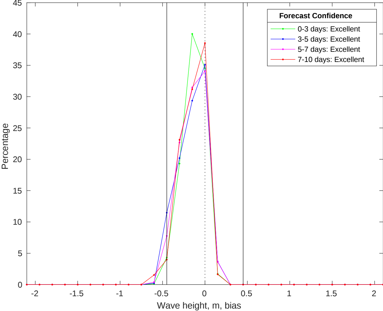
NDBC 52212 vs CMEMS Waves Bias Histogram: 04-Jun-2025
