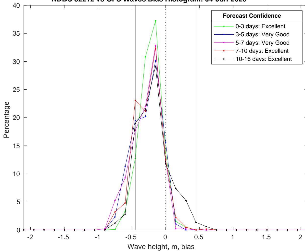
NDBC 52212 vs GFS Waves Bias Histogram: 04-Jun-2025
