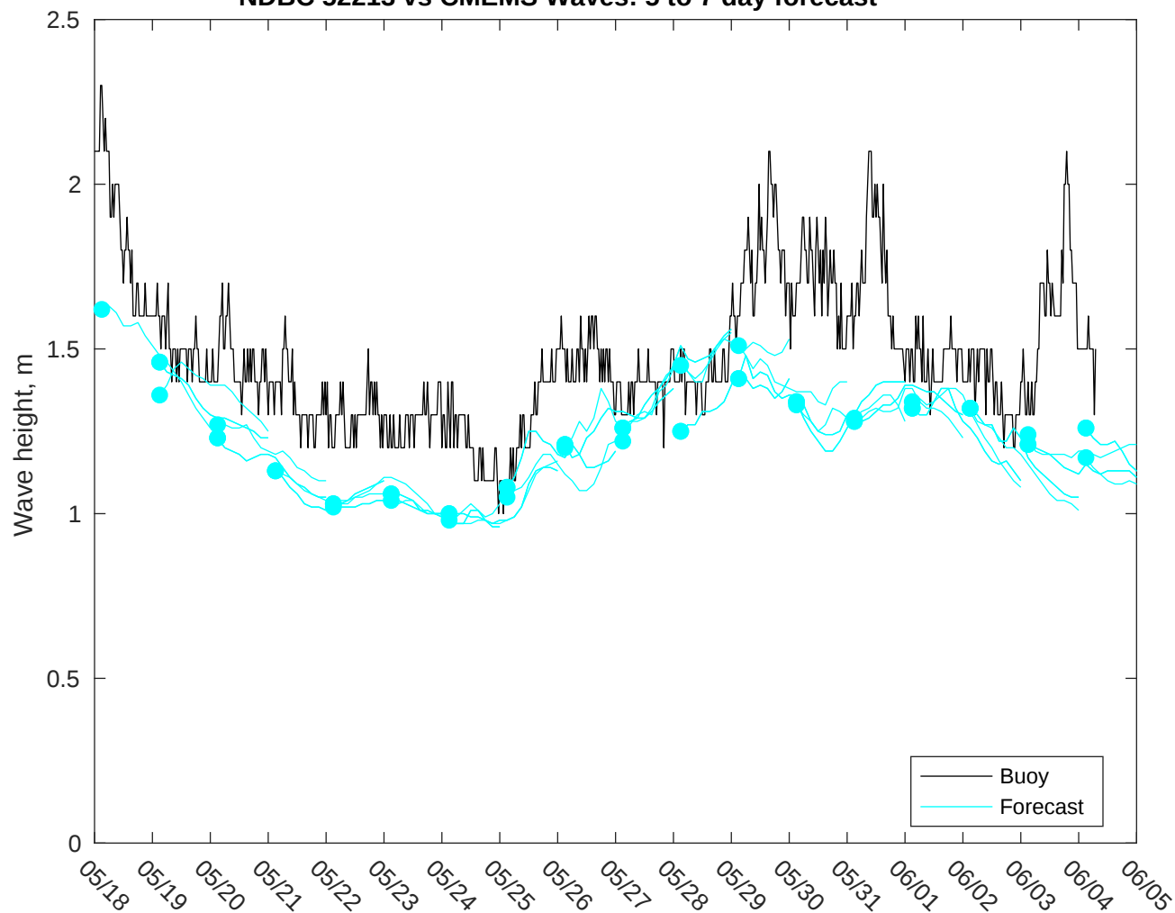
NDBC 52213 vs CMEMS Waves: 5 to 7 day forecast
