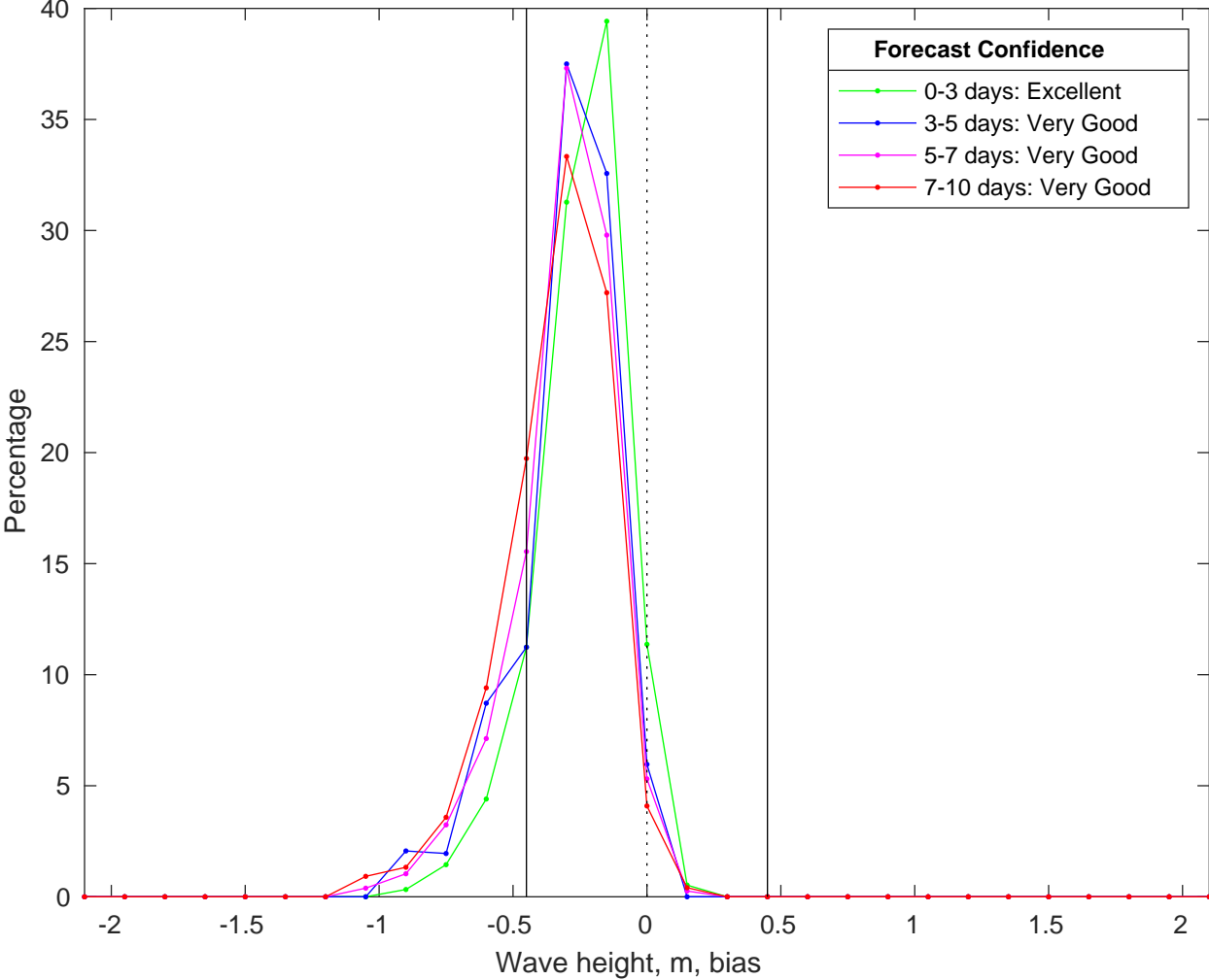
NDBC 52213 vs CMEMS Waves Bias Histogram: 04-Jun-2025
