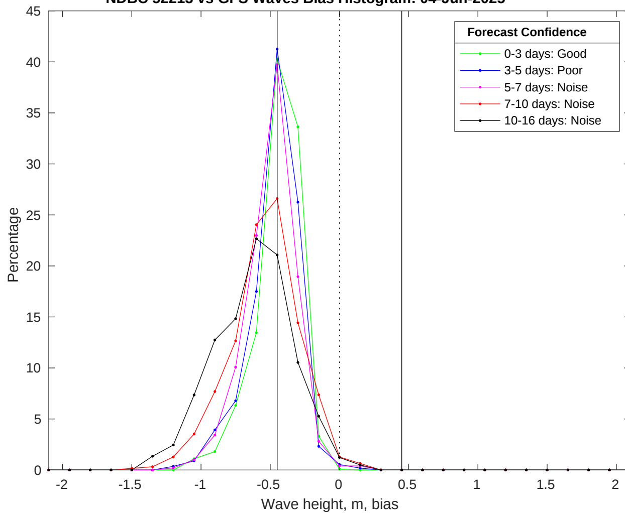
NDBC 52213 vs GFS Waves Bias Histogram: 04-Jun-2025
